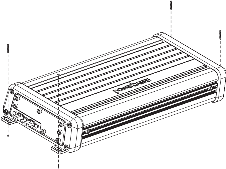
Fig.1 Mounting Amplifier
