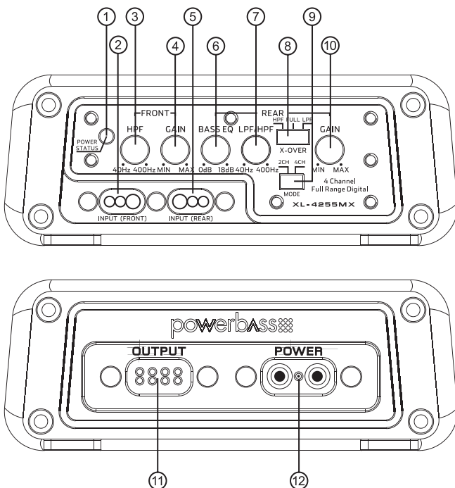
Fig.3 4-Channel Panel Layout
