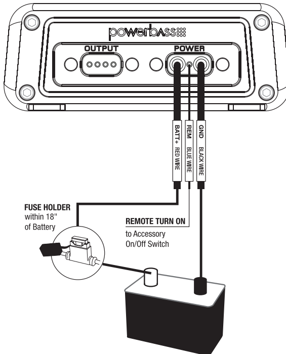
Fig.7 Proper Ground Connection For UTVs, Motorcycles or Boats
