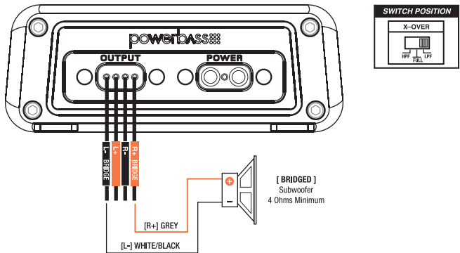
Fig.18 1-CH (Bridged Mode) Speaker Connection (Do not connect total impedance under 4 ohms)
