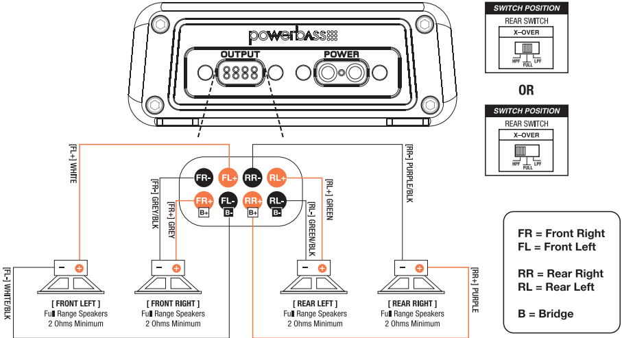
Fig.19 4-CH Speaker Connection / 2 ohms minimum
