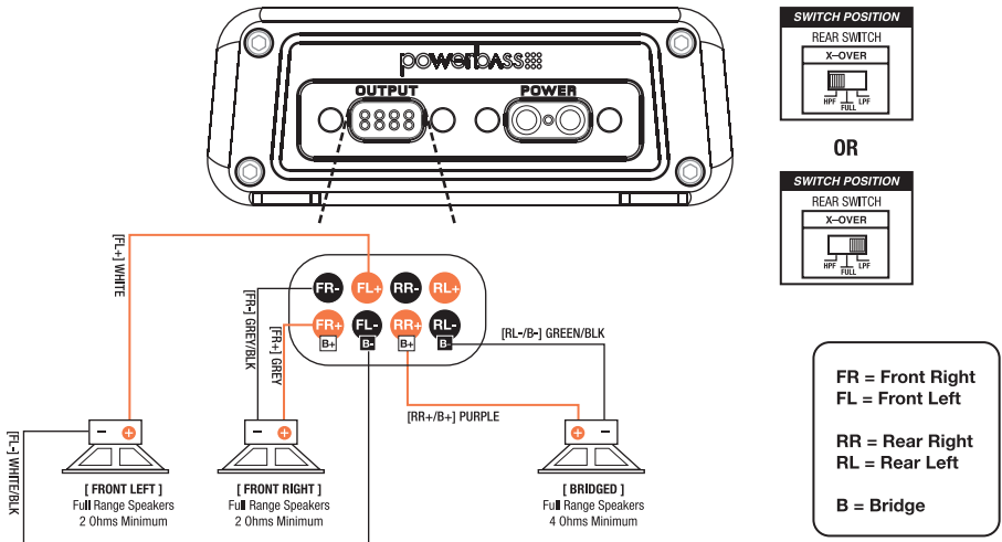
Fig.20 3-CH Speaker Connection
