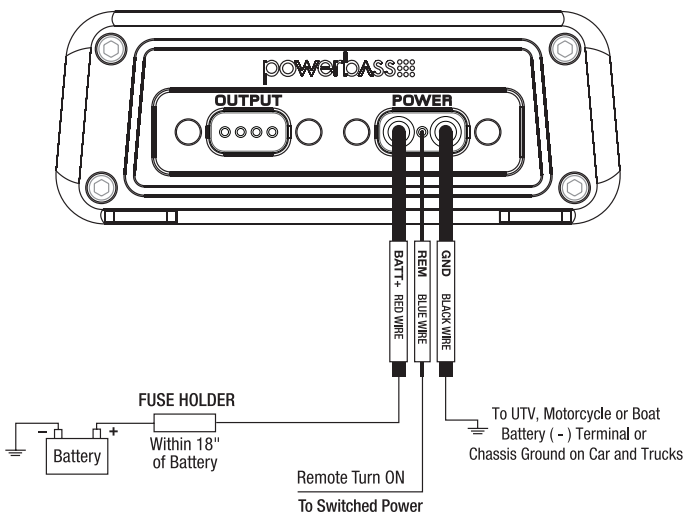
Fig.5 Power Input Connection
