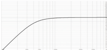
Sealed (Maximum)
