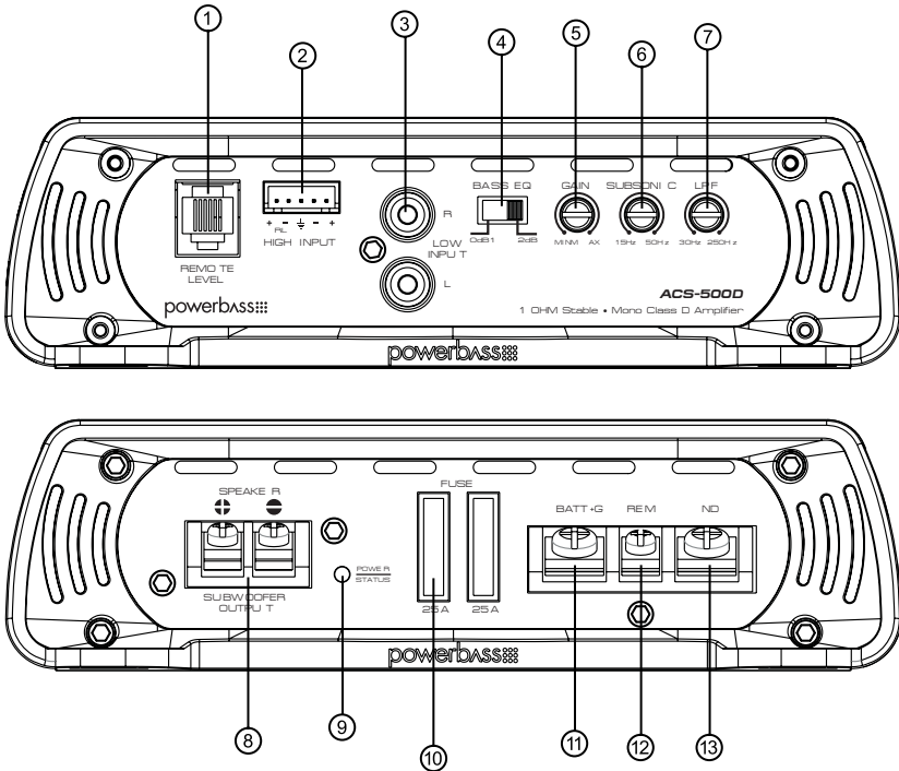
Fig.2 Panel Layout
